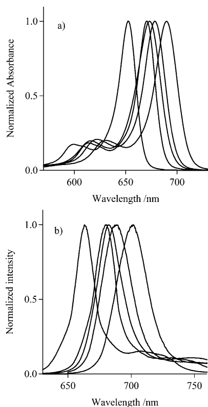
Figure 4. a) Normalized absorption and b) fluorescence spectra of (from left to right) KFL-3, KFL-5, KFL-6, KFL-9, and KFL-10 in chloroform.
