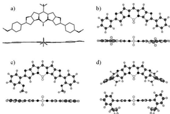
Figure 2. a) X-ray molecular structure of KFL-4 [31] and AM1 calculated molecular structures of b) KFL-5, c) KFL-6, and d) KFL-8. Top figures and bottom figures in each dye represent front view and side view, respectively.
