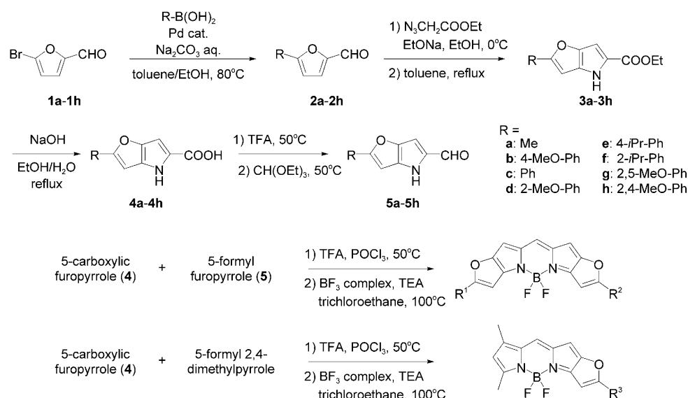
Scheme 1. Synthetic scheme for Keio Fluors.
