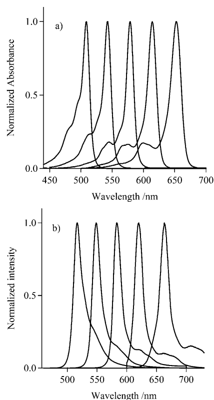
Figure 5. a) Normalized absorption and b) fluorescence spectra of (from left to right) TM-BDP, KFL-11, KFL-1, KFL-12, and KFL-5 in chloroform.
