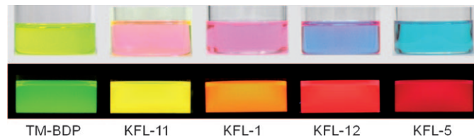
Figure 6. Absorption (upper row) and fluorescence (bottom row) colors of TM-BDP and KFLs in chloroform.
