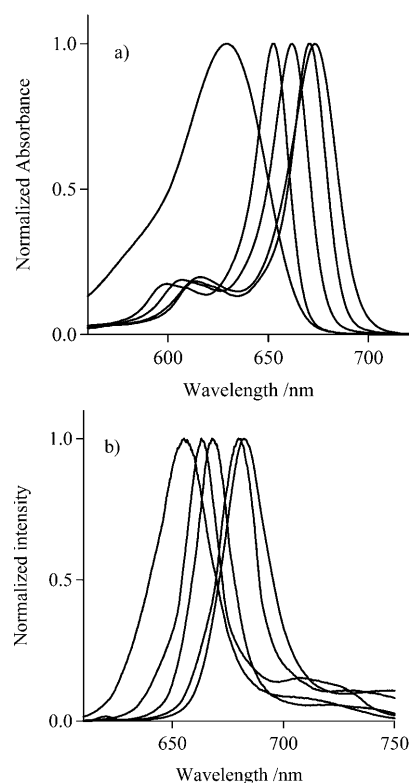
Figure 1. a) Normalized absorption and b) fluorescence spectra of (from left to right) KFL-3 and KFL-5–8 in chloroform.
