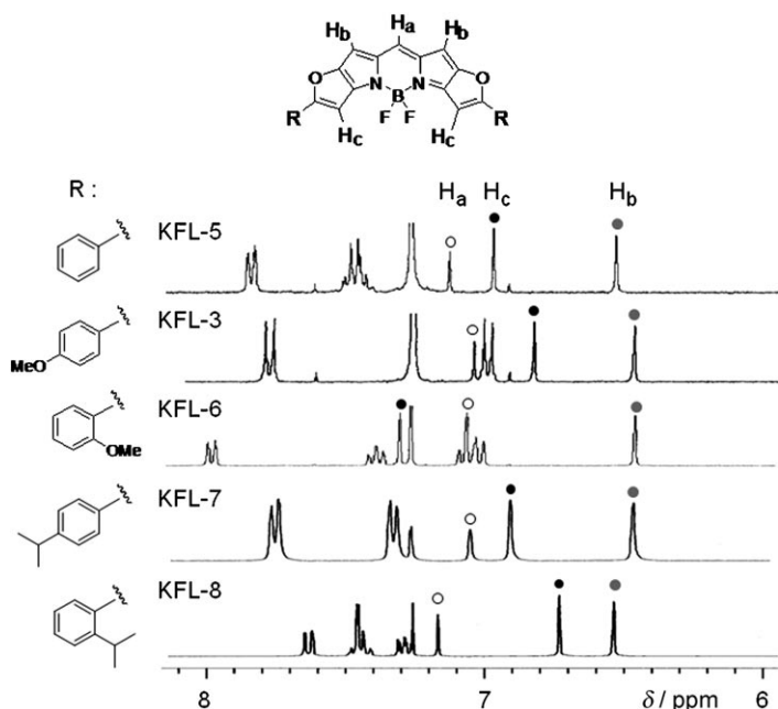
Figure 3. NMR spectra of KFL-3 and KFL-5-8 in [D 1 ]chloroform at room temperature.
